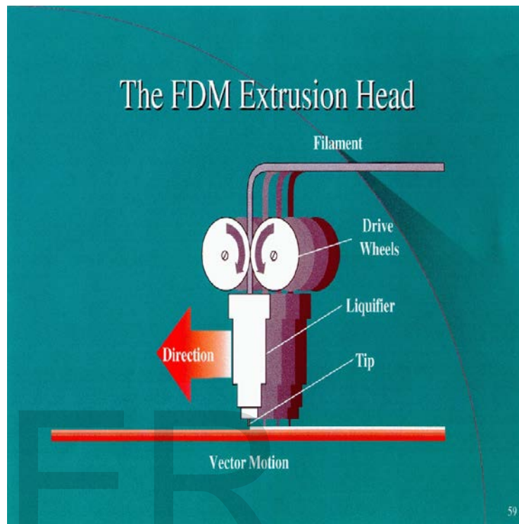
Figure 4: Schematic diagram of fused deposition modeling.
