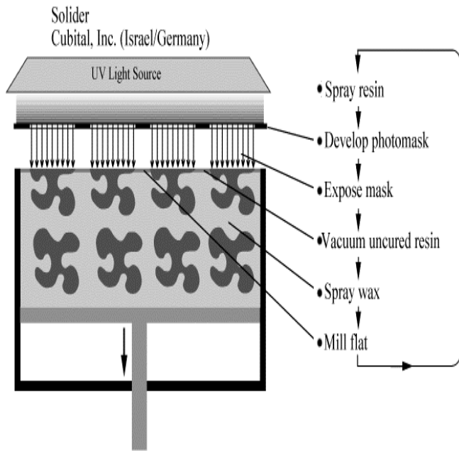
Figure 5: Schematic diagram of solid ground curing.
