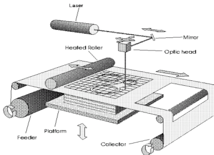
Figure 2: Schematic diagram of laminated object manufacturing.
